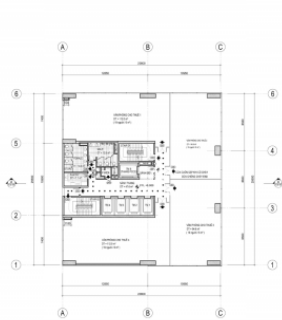
Typical ground plan
