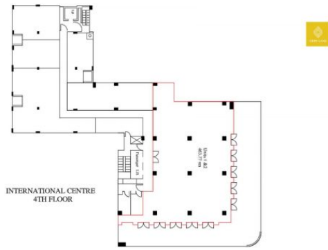
Floor plan 4
