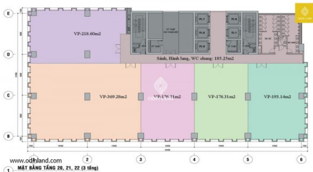
Floor plan of the 20th floor; 21; 22 (3 floors)
