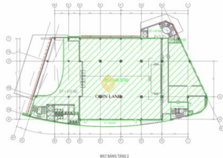
2nd floor plan of The Manor Palace building
