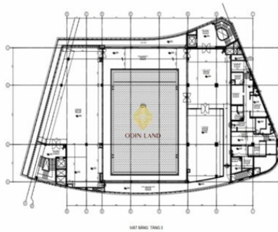
3rd floor plan of The Manor Palace building
