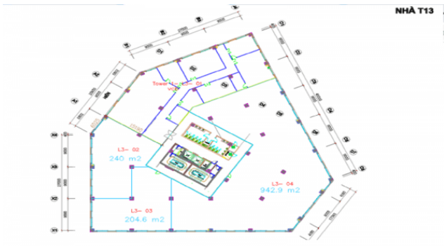
Floor plan of Tower 1 building
