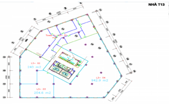
Floor plan of Tower 1 building
