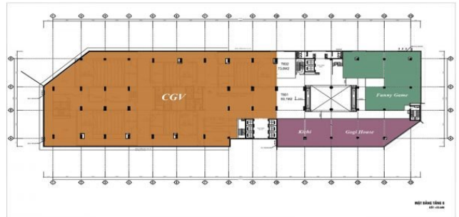
Floor plan of Artemis building - Floor 6
